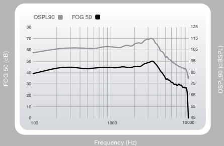
OSPL90 (gray) and Full-On Gain (black) curves for the Halo 2 RIC 13 at 115/50.
