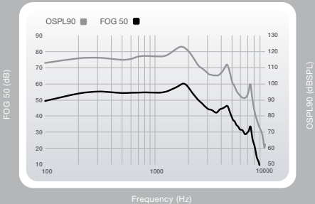
OSPL90 (gray) and Full-On Gain (black) curves for the Halo 2 RIC 13 AP at 123/60.
