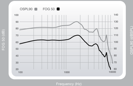
OSPL90 (gray) and Full-On Gain (black) curves for the Halo 2 RIC 13 AP at 130/70.
