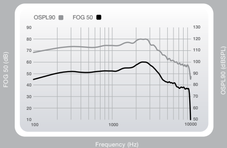
OSPL90 (gray) and Full-On Gain (black) curves for the Halo 2 RIC 13 at 120/60.
